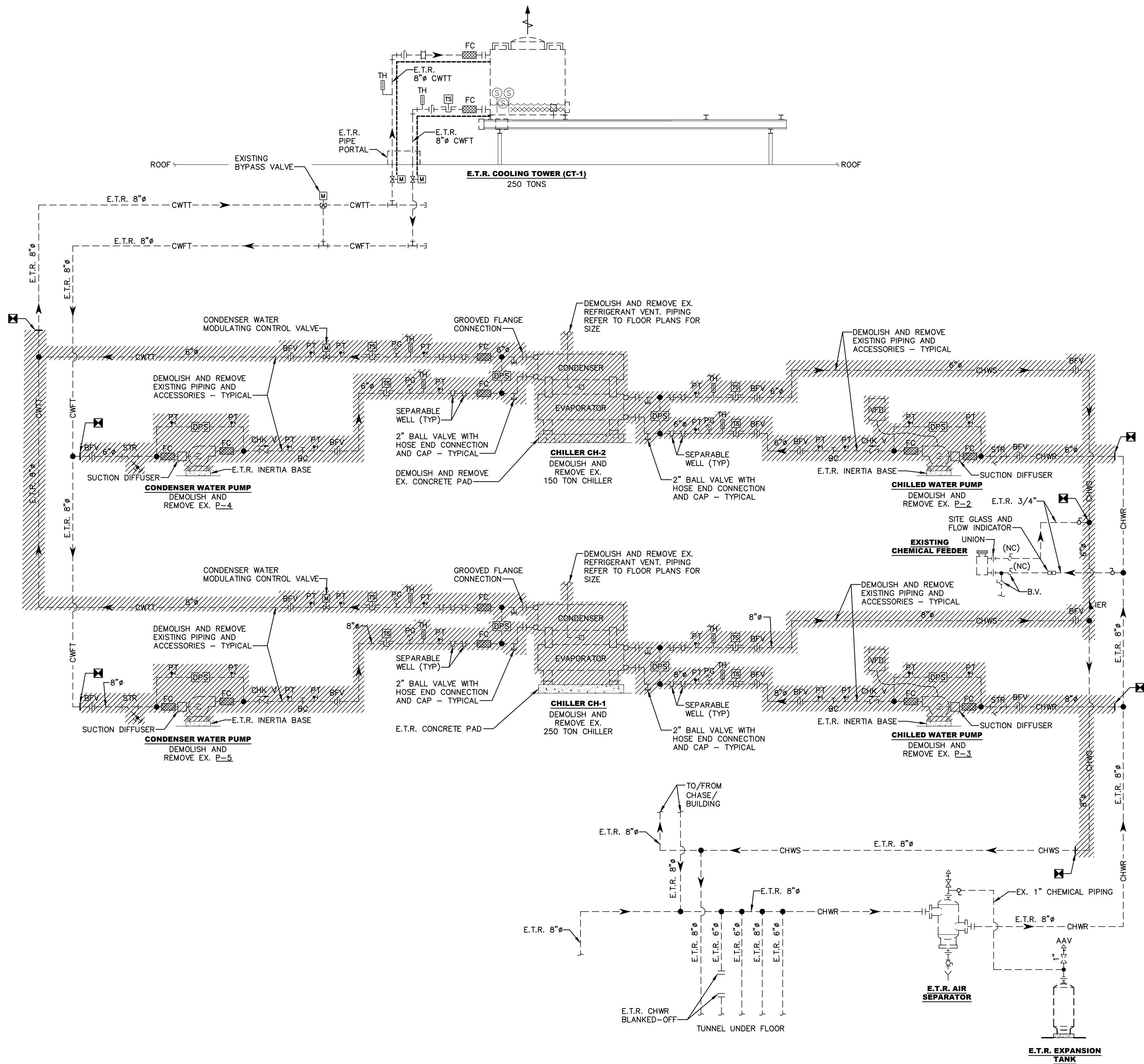
CHILLED AND CONDENSER WATER SCHEMATIC FLOW DIAGRAM - HVAC DEMOLITION
