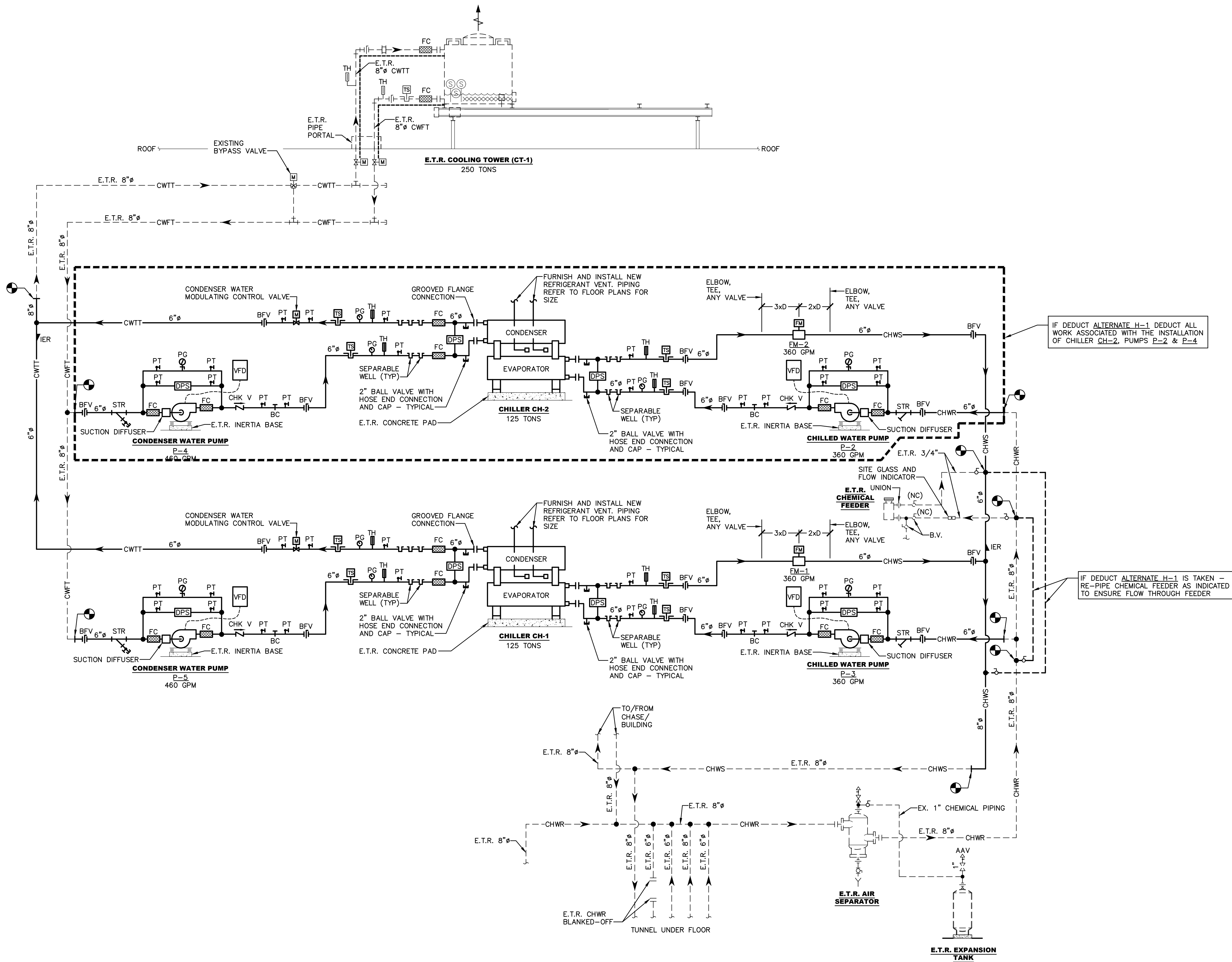
CHILLED AND CONDENSER WATER SCHEMATIC FLOW DIAGRAM - HVAC NOT TO SCALE
